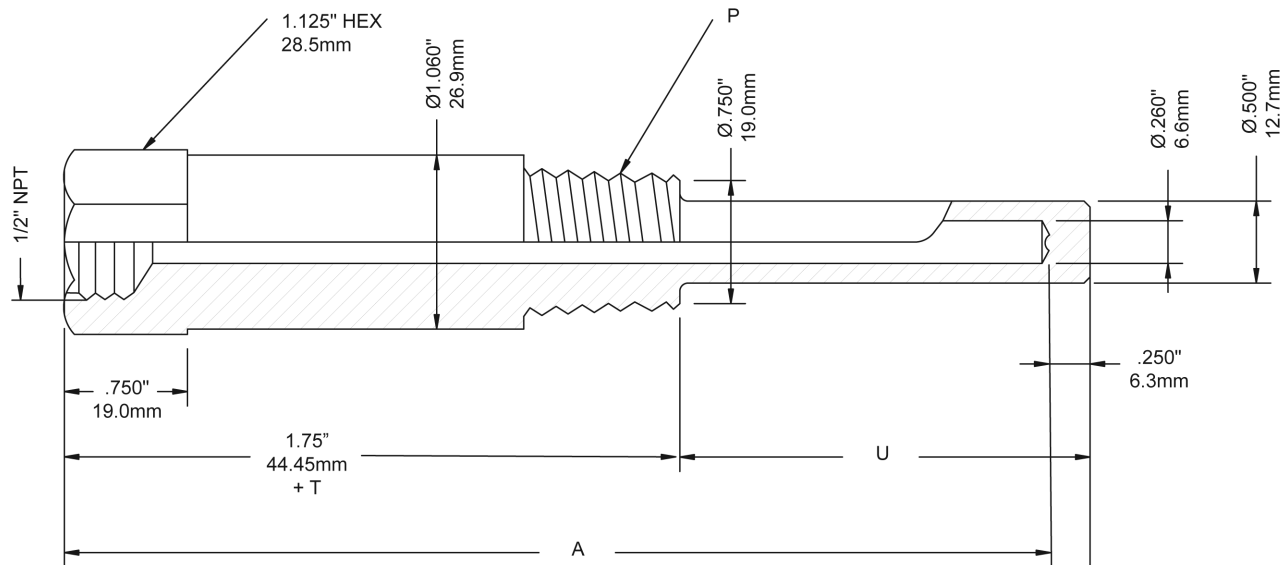
Standard Thermowell with lag
